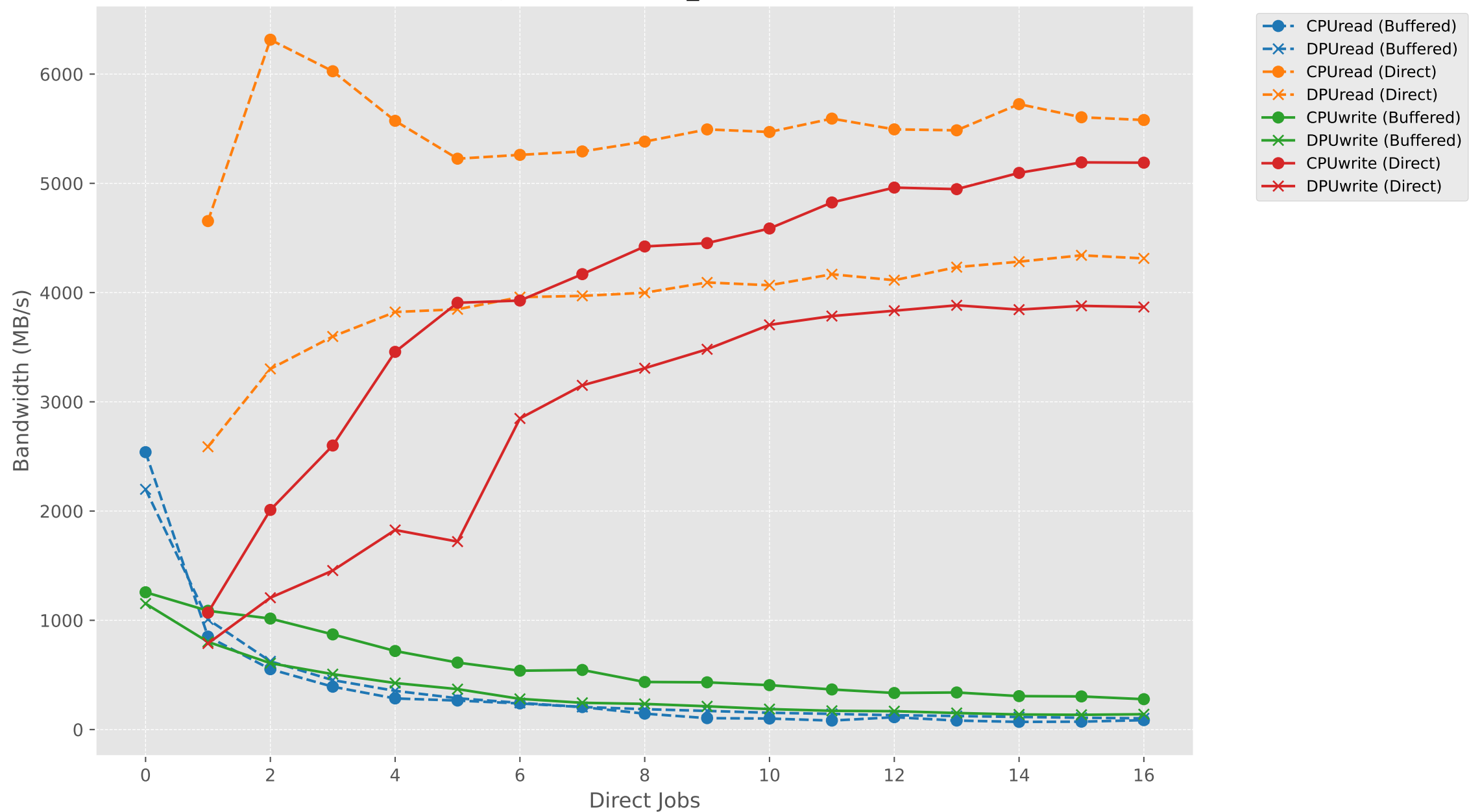
Bandwidth vs Direct Jobs (buffered1_directN) - SEQ (CPU vs DPU)
